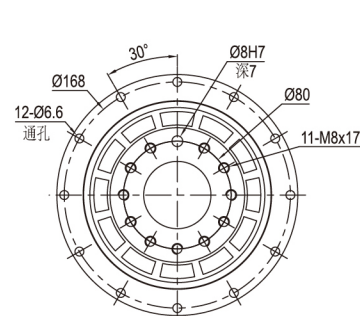
输出端/OUTPUT
