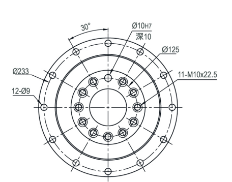
输出端/OUTPUT
